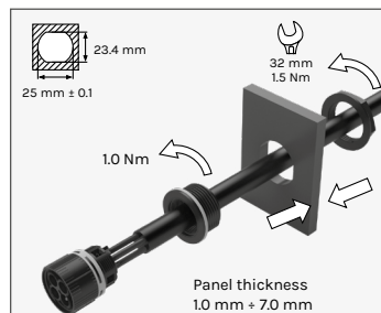
PANEL FIXING DETAILS M25
