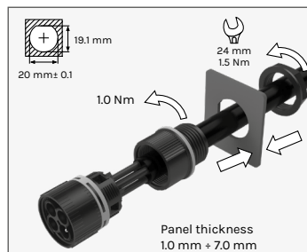
PANEL FIXING DETAILS M20
