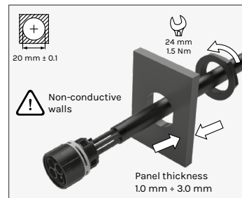
PANEL FIXING DETAILS M20 (N.C.)
